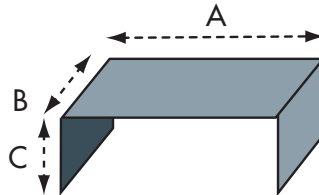
Type 2 Covering altar mensa with side drops Total length = A + 2xC Total depth = B
